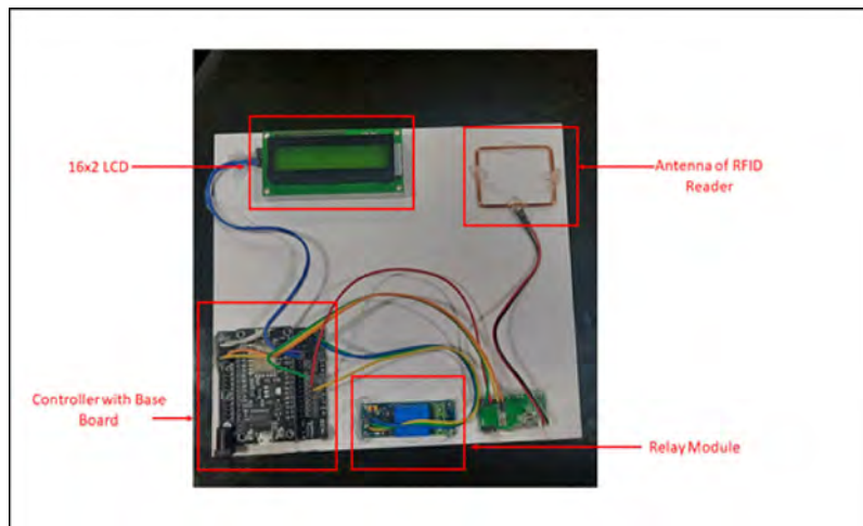
Figure 2 – Hardware Setup
